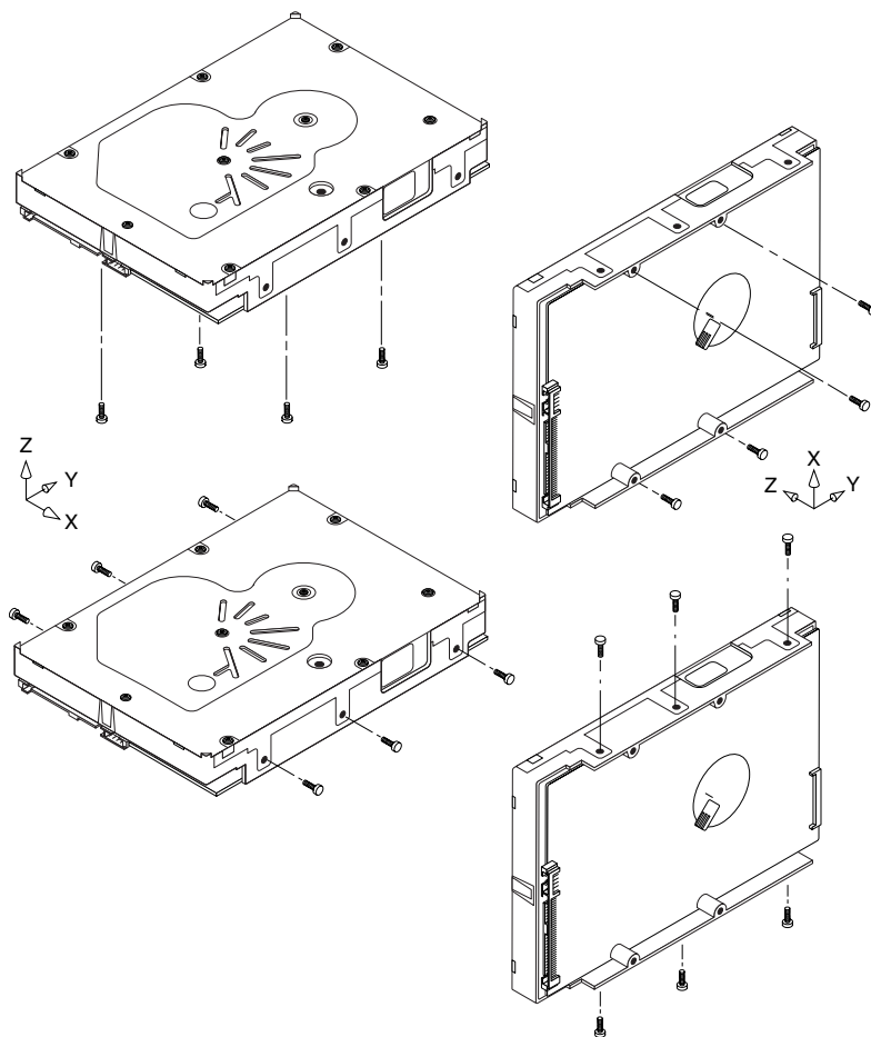
Figure 6. Recommended mounting
