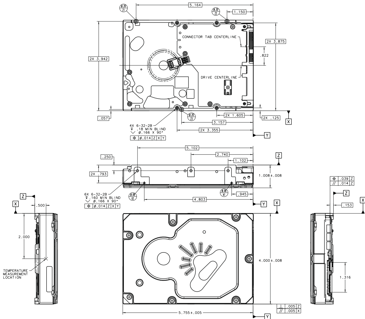
Figure 7. Physical dimensions
