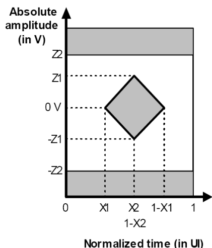
Figure 14. Receive eye mask
