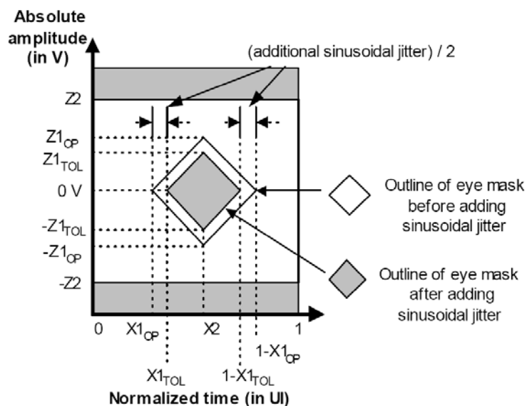
Figure 15. Receive tolerance eye mask
