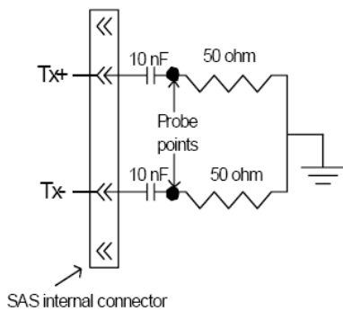
Figure 18. Zero-length test load
